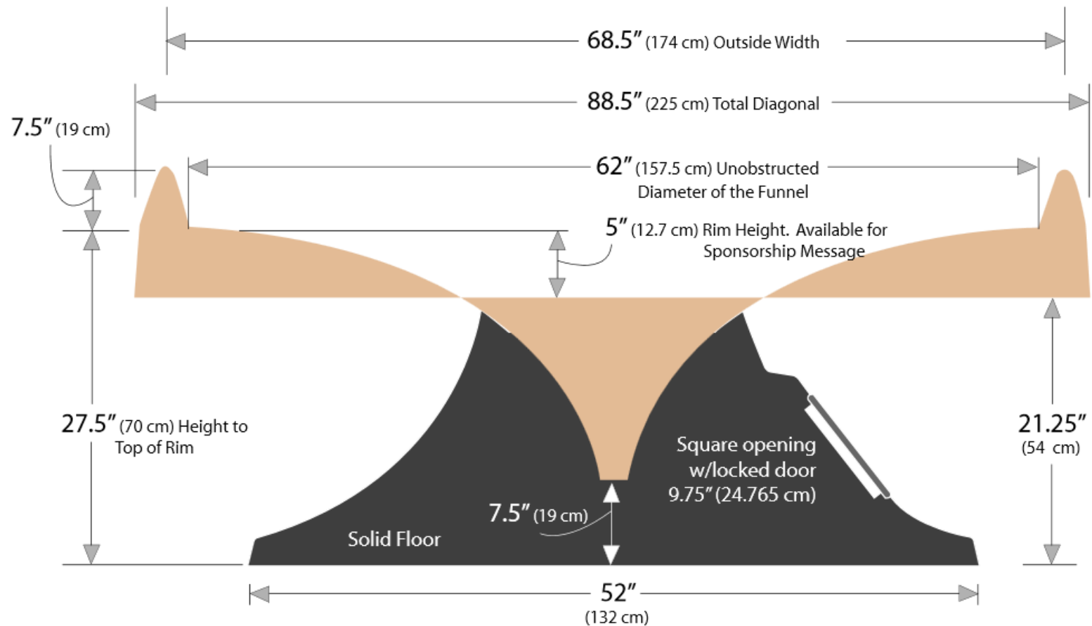
Seven-Footer Spiral Wishing Well – Detailed Dimensions www.SpiralWishingWells.com
